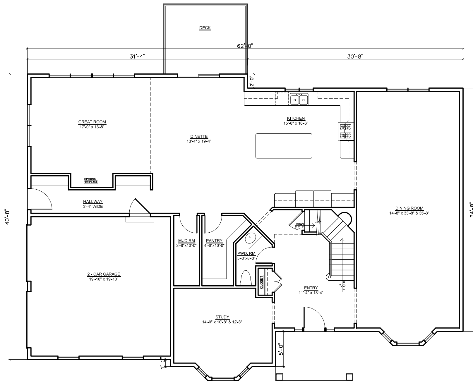
MAIN FLOOR PLAN 1980 SQ.FT. + 413 SQ.FT. GARAGE
