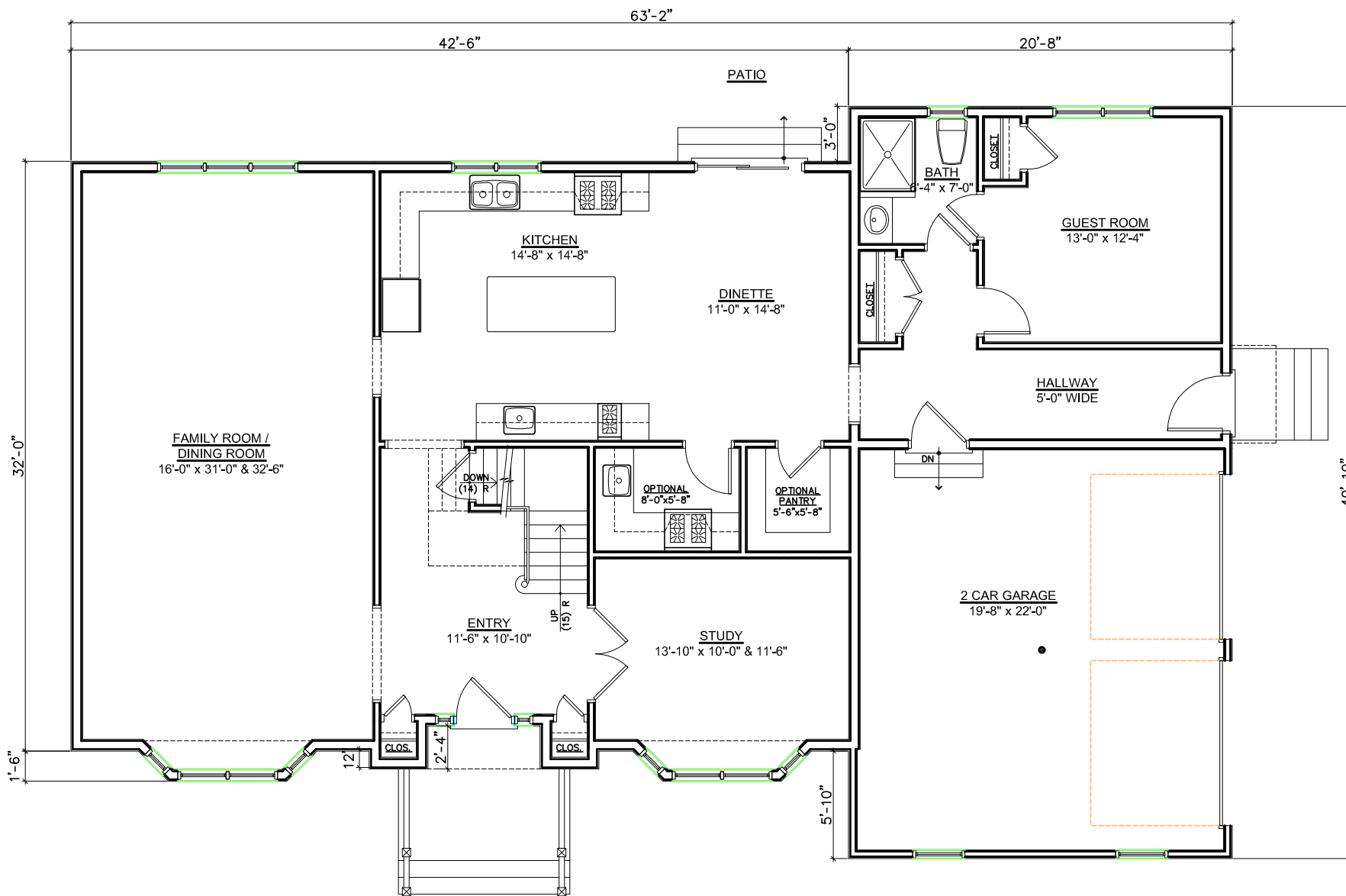
MAIN FLOOR PLAN 1775 SQ.FT.
