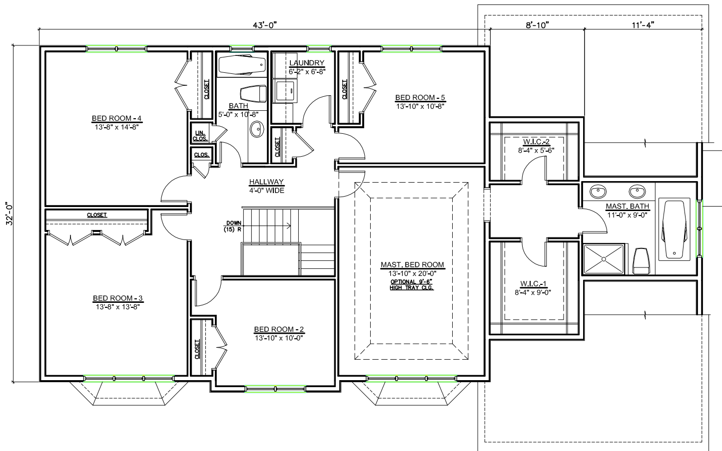
SECOND FLOOR PLAN 1634 SQ.FT.
